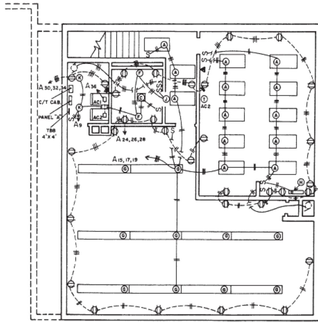
BASEMENT LIGHTING AND POWER PLAN SCALE 1/8" = 1'-0"
